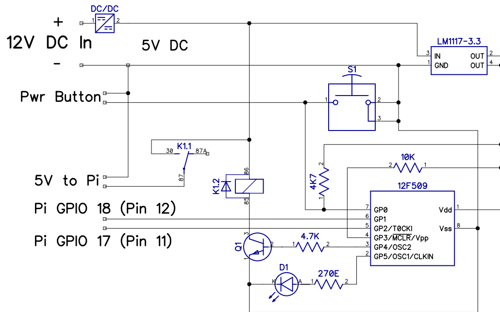
RetroPi Power Supply Controller
